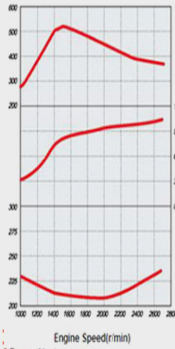
Power Curve
